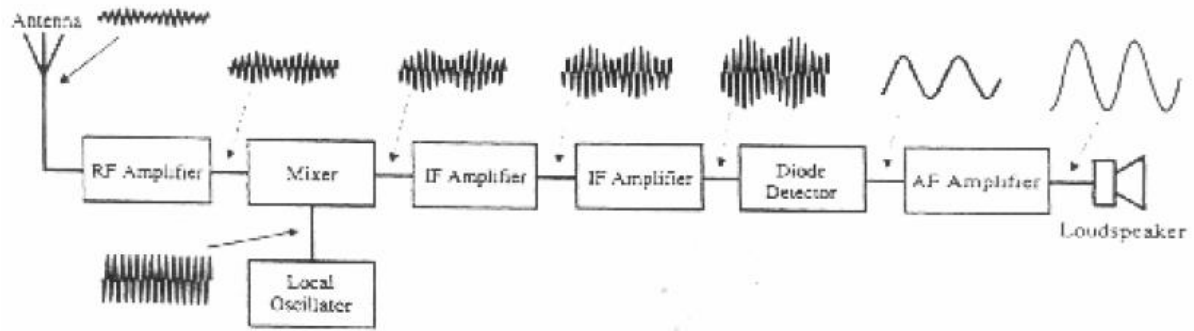
Figure 3: AM Reception
