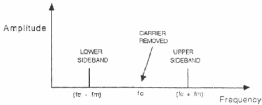
Figure 3: DSBSC Sidebands
